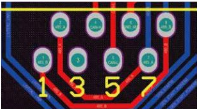
CANBus Port
